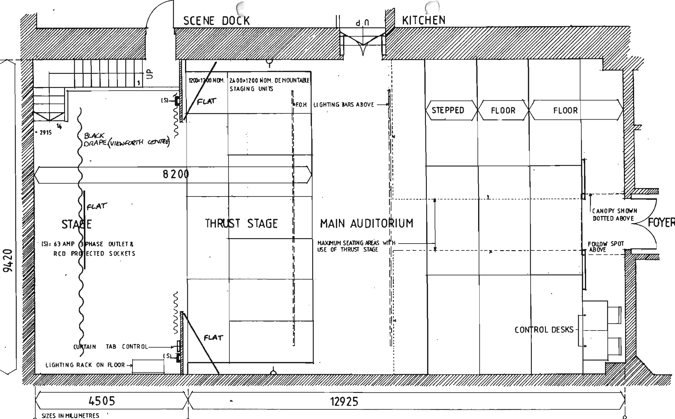
VIEWFORTH CENTRE MAIN AUDITORIUM FLOOR PLAN 3
